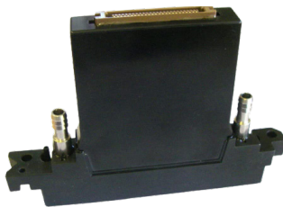
KM1024i PrinterHead
